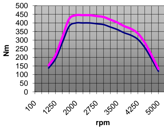
Torque
